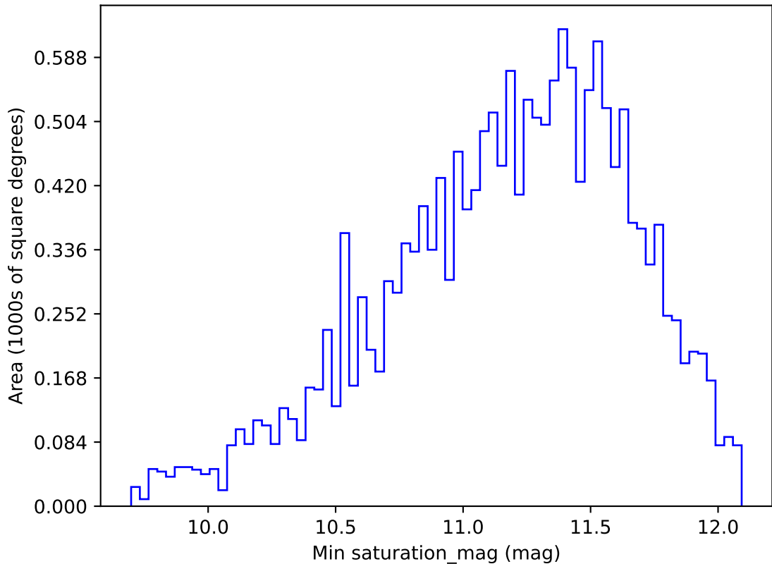
ddf_loaded_half_fl1_v3.4_10yrs WFD y band: Min saturation_mag
