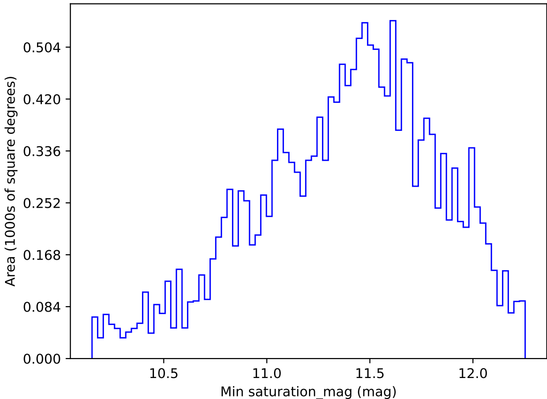
ddf_loaded_half_fl1_v3.4_10yrs WFD u band: Min saturation_mag
