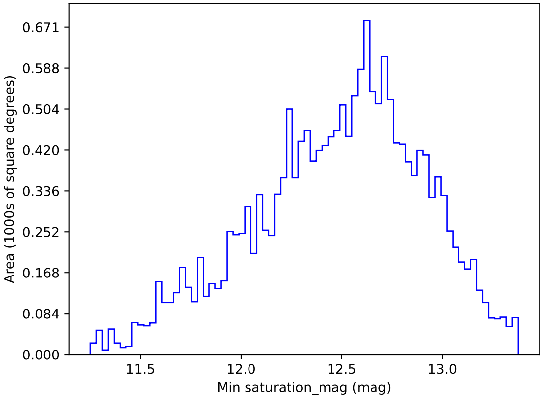
ddf_loaded_half_fl1_v3.4_10yrs WFD r band: Min saturation_mag
