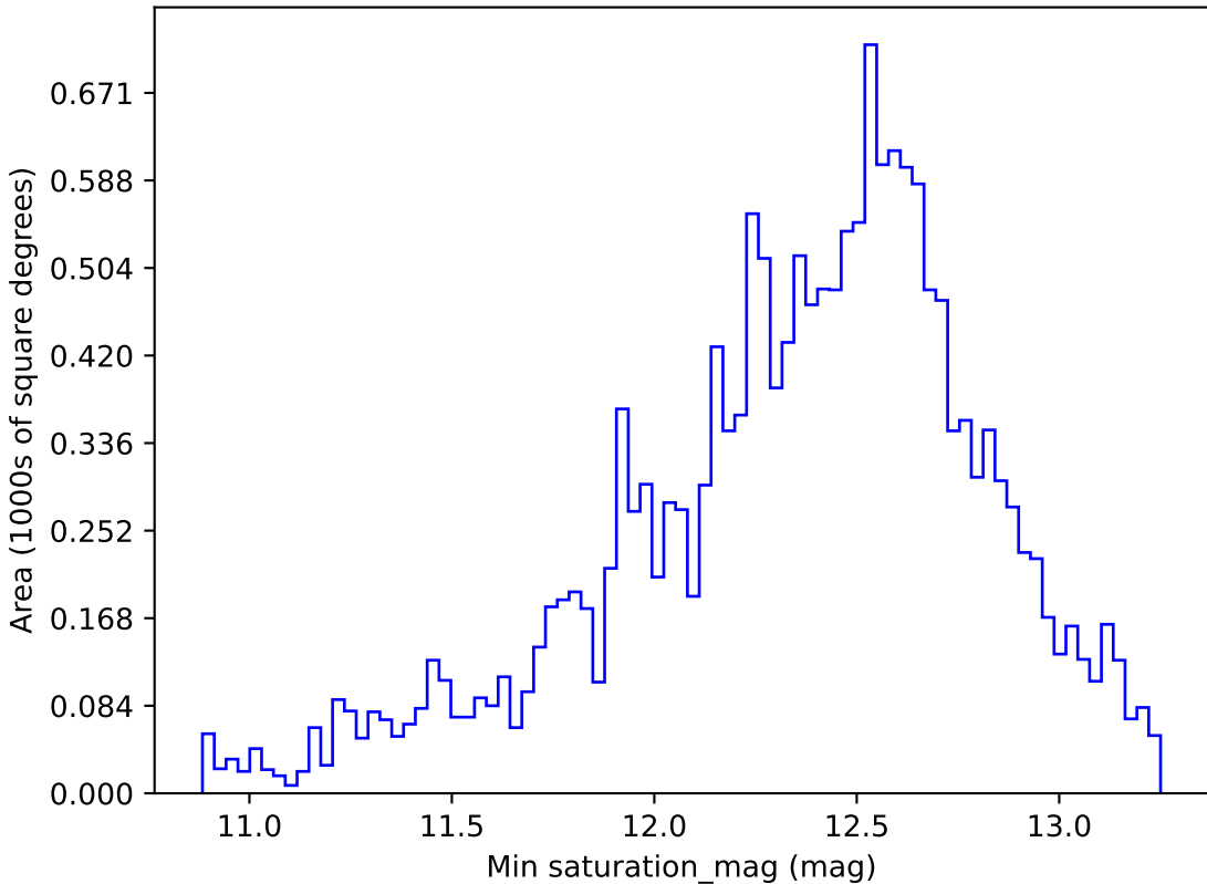
ddf_loaded_half_fl1_v3.4_10yrs WFD i band: Min saturation_mag
