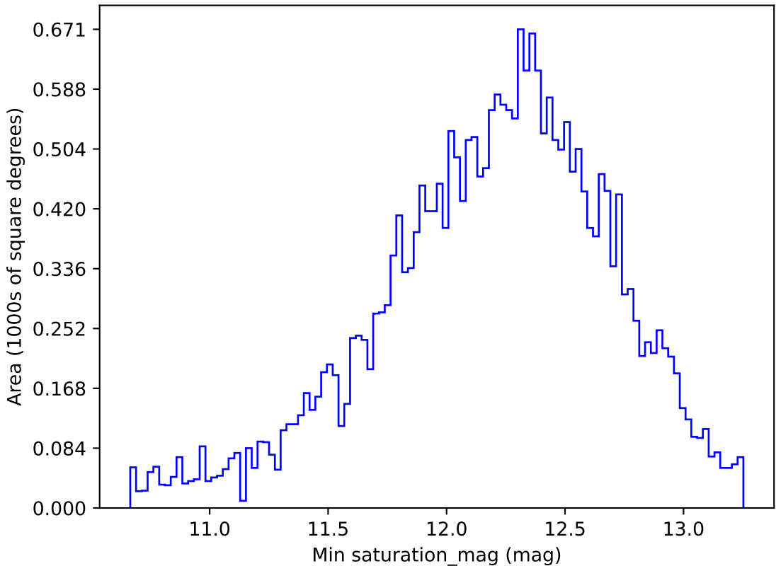
ddf_loaded_half_fl1_v3.4_10yrs All sky z band: Min saturation_mag
