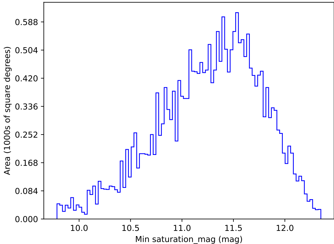
ddf_loaded_half_fl1_v3.4_10yrs All sky y band: Min saturation_mag
