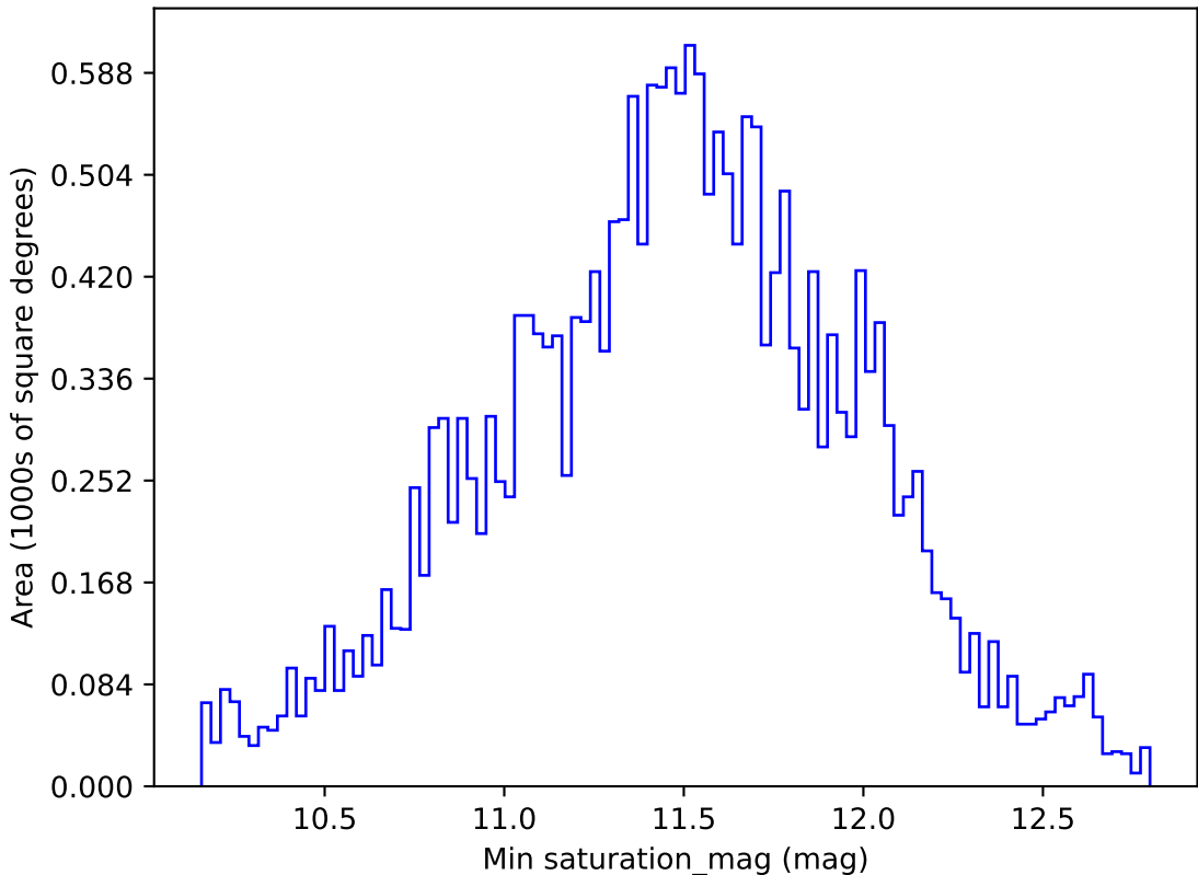
ddf_loaded_half_fl1_v3.4_10yrs All sky u band: Min saturation_mag
