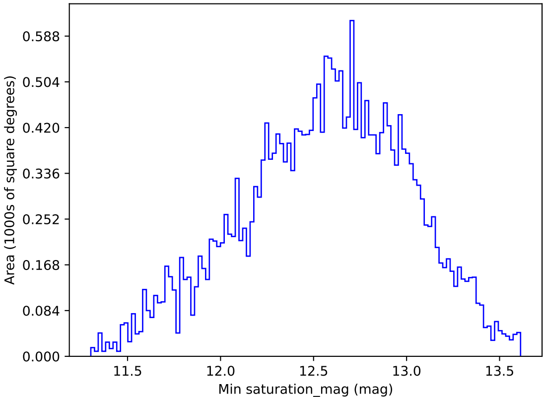
ddf_loaded_half_fl1_v3.4_10yrs All sky r band: Min saturation_mag
