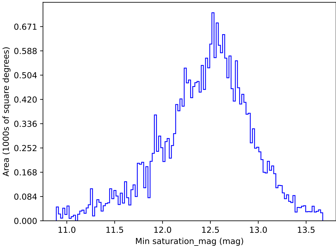
ddf_loaded_half_fl1_v3.4_10yrs All sky i band: Min saturation_mag
