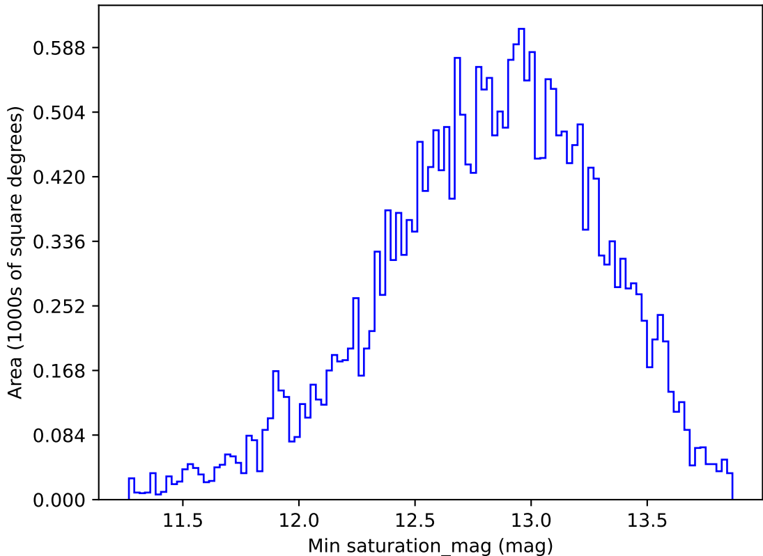
ddf_loaded_half_fl1_v3.4_10yrs All sky g band: Min saturation_mag
