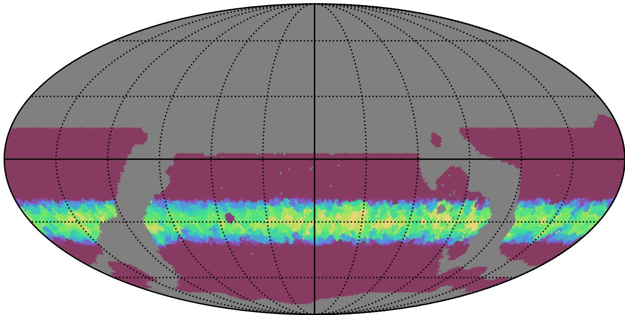
ddf_loaded_half_fl1_v3.4_10yrs WFD z band: Min normairmass
