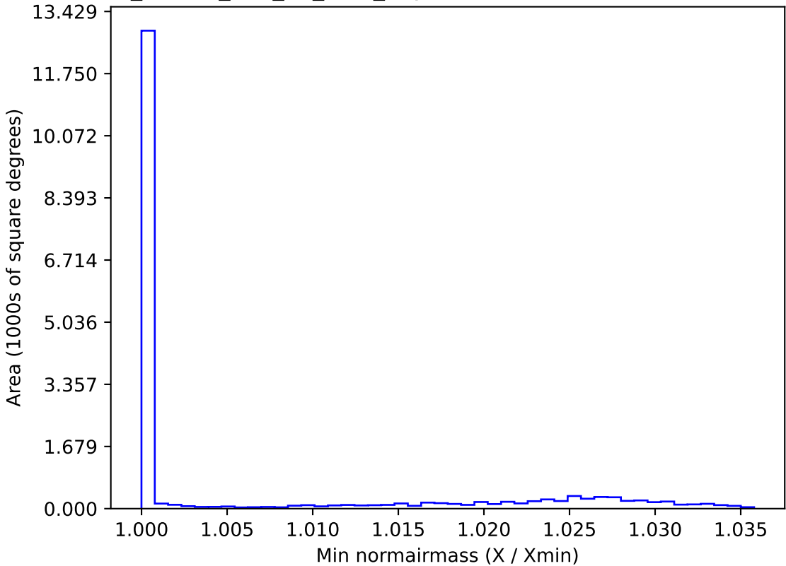
ddf_loaded_half_fl1_v3.4_10yrs WFD z band: Min normairmass
