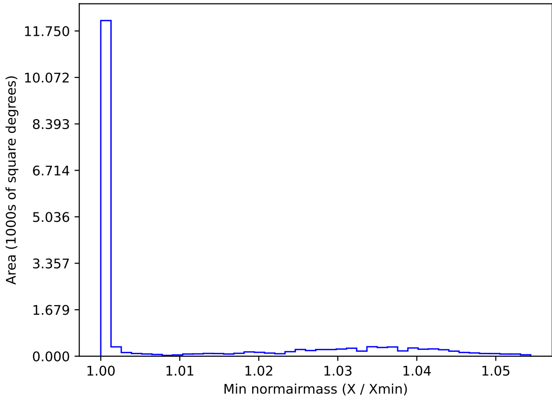
ddf_loaded_half_fl1_v3.4_10yrs WFD u band: Min normairmass
