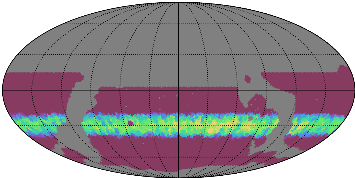
ddf_loaded_half_fl1_v3.4_10yrs WFD r band: Min normairmass
