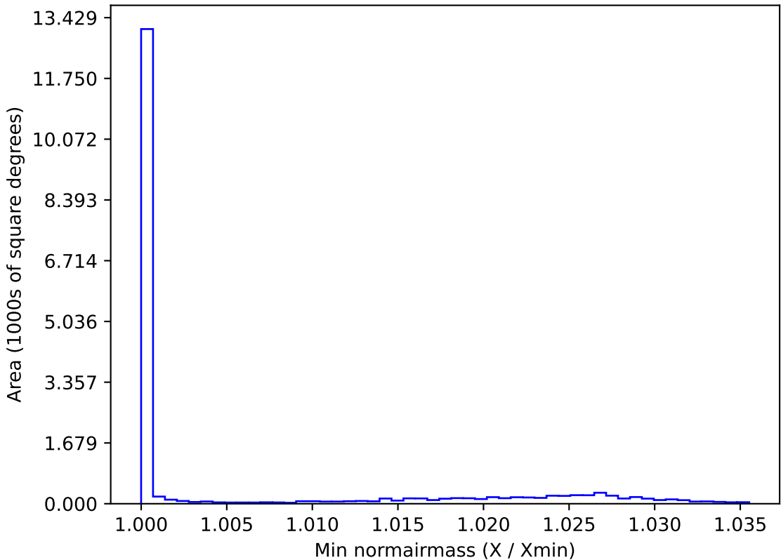
ddf_loaded_half_fl1_v3.4_10yrs WFD r band: Min normairmass
