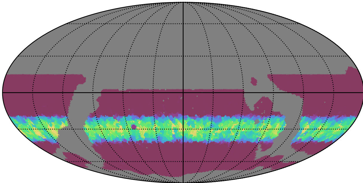
ddf_loaded_half_fl1_v3.4_10yrs WFD g band: Min normairmass
