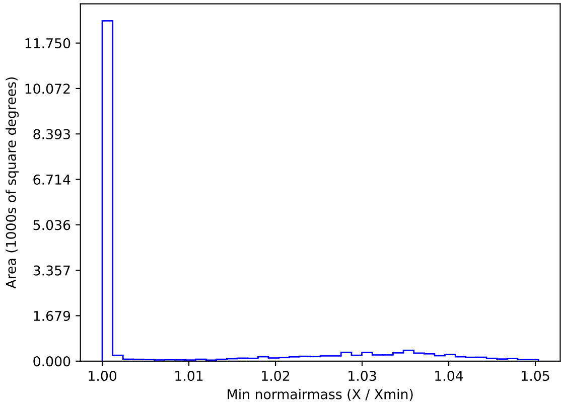
ddf_loaded_half_fl1_v3.4_10yrs WFD g band: Min normairmass
