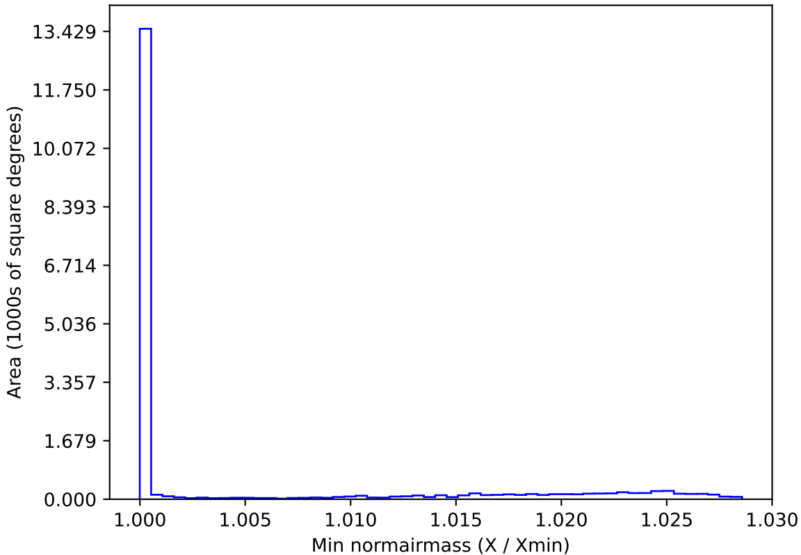
ddf_loaded_half_fl1_v3.4_10yrs WFD all bands: Min normairmass
