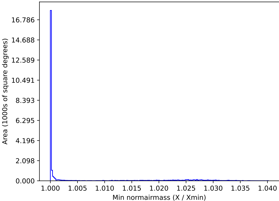
ddf_loaded_half_fl1_v3.4_10yrs All sky z band: Min normairmass
