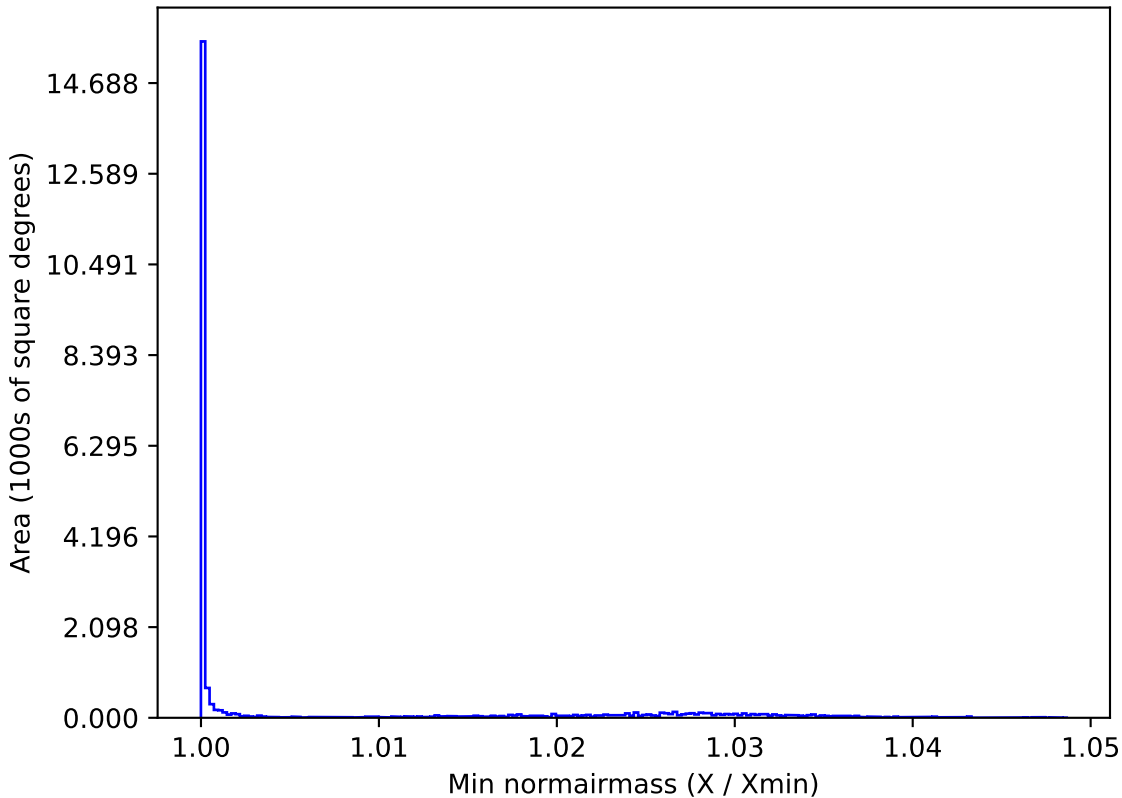
ddf_loaded_half_fl1_v3.4_10yrs All sky y band: Min normairmass
