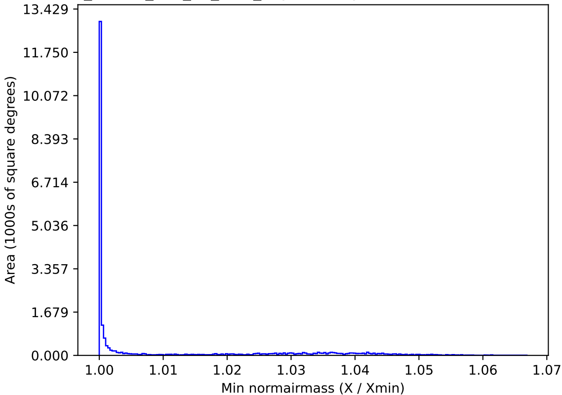
ddf_loaded_half_fl1_v3.4_10yrs All sky u band: Min normairmass
