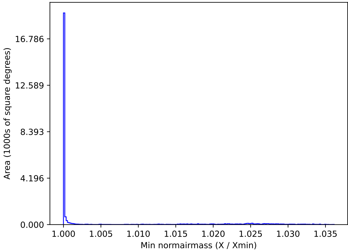
ddf_loaded_half_fl1_v3.4_10yrs All sky i band: Min normairmass
