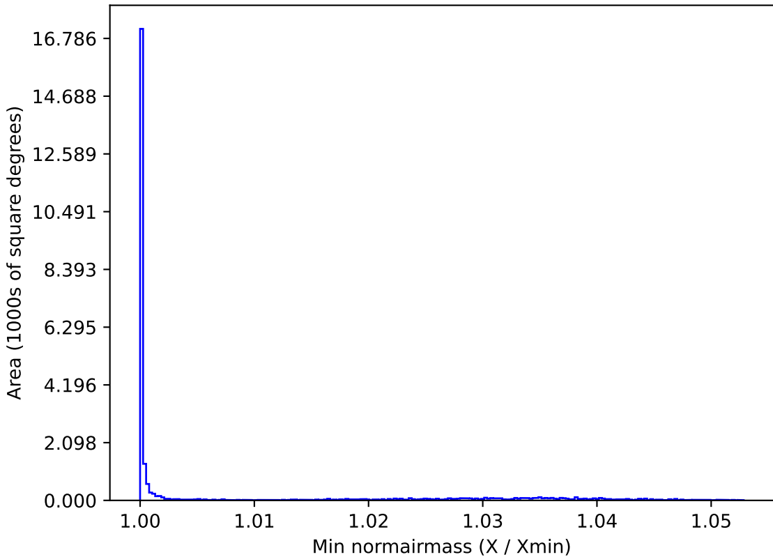
ddf_loaded_half_fl1_v3.4_10yrs All sky g band: Min normairmass
