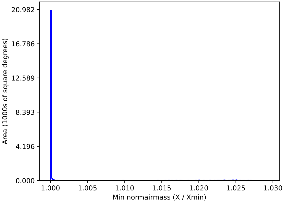
ddf_loaded_half_fl1_v3.4_10yrs All sky all bands: Min normairmass
