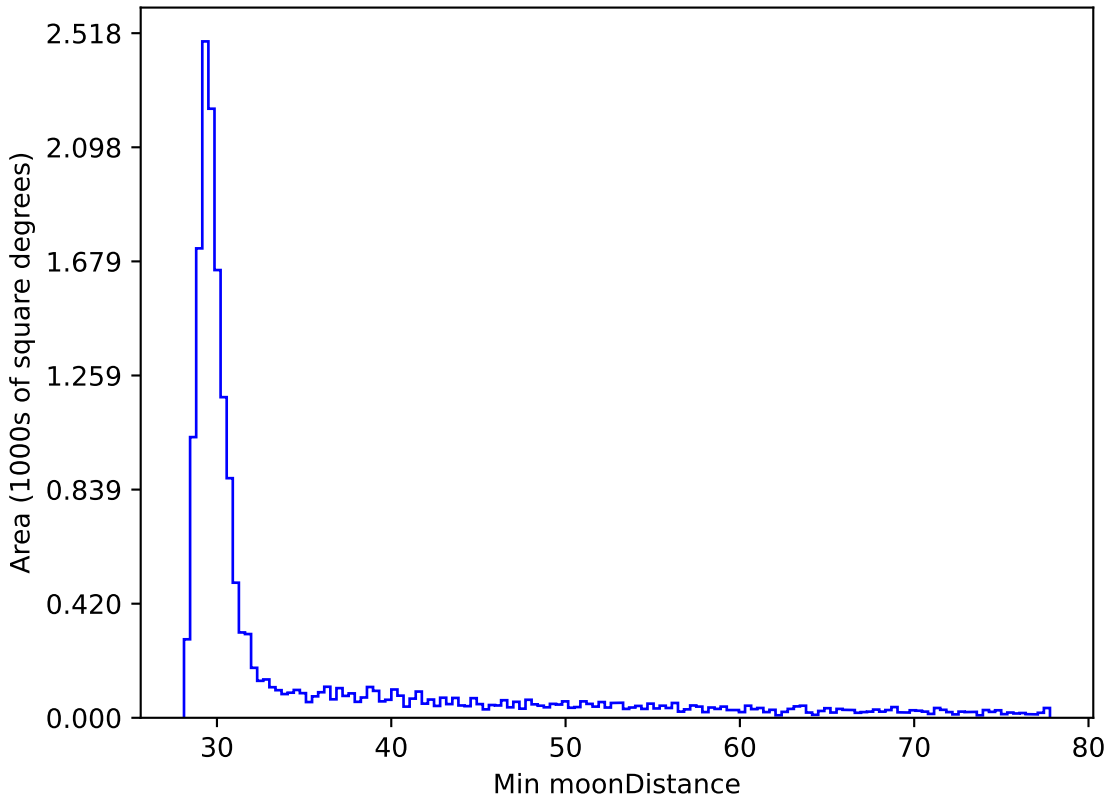
ddf_loaded_half_fl1_v3.4_10yrs WFD z band: Min moonDistance
