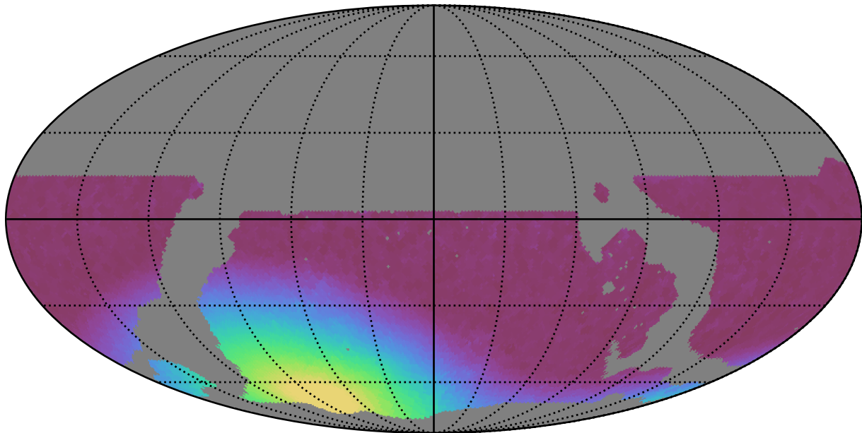
ddf_loaded_half_fl1_v3.4_10yrs WFD y band: Min moonDistance
