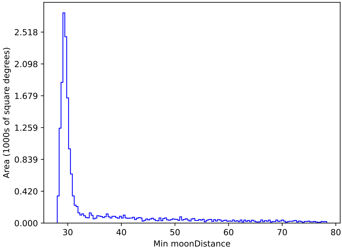
ddf_loaded_half_fl1_v3.4_10yrs WFD y band: Min moonDistance
