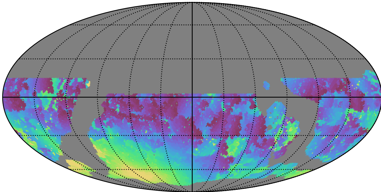
ddf_loaded_half_fl1_v3.4_10yrs WFD u band: Min moonDistance
