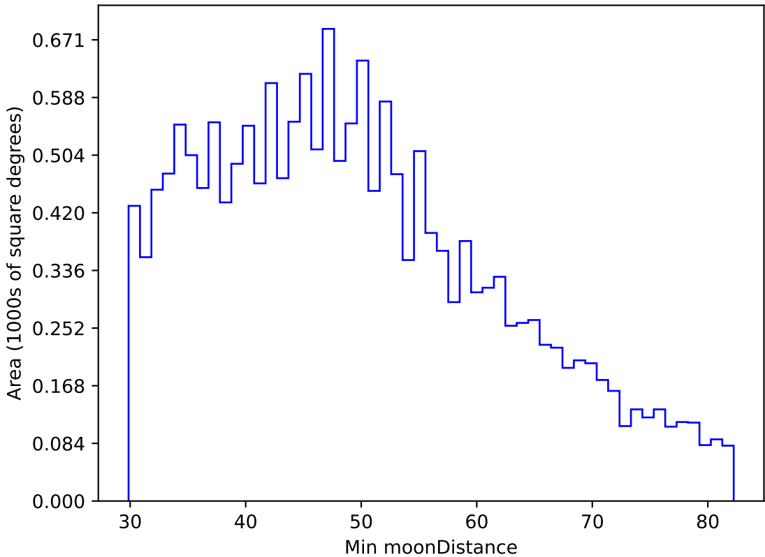
ddf_loaded_half_fl1_v3.4_10yrs WFD u band: Min moonDistance
