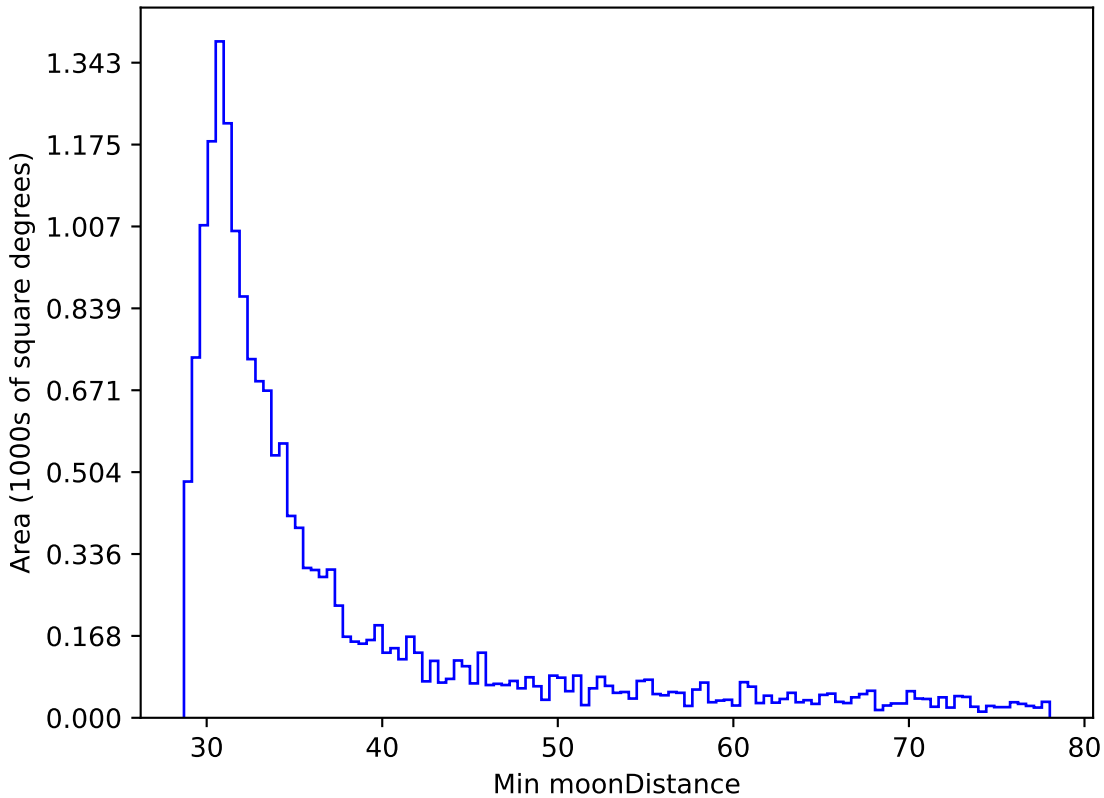
ddf_loaded_half_fl1_v3.4_10yrs WFD r band: Min moonDistance
