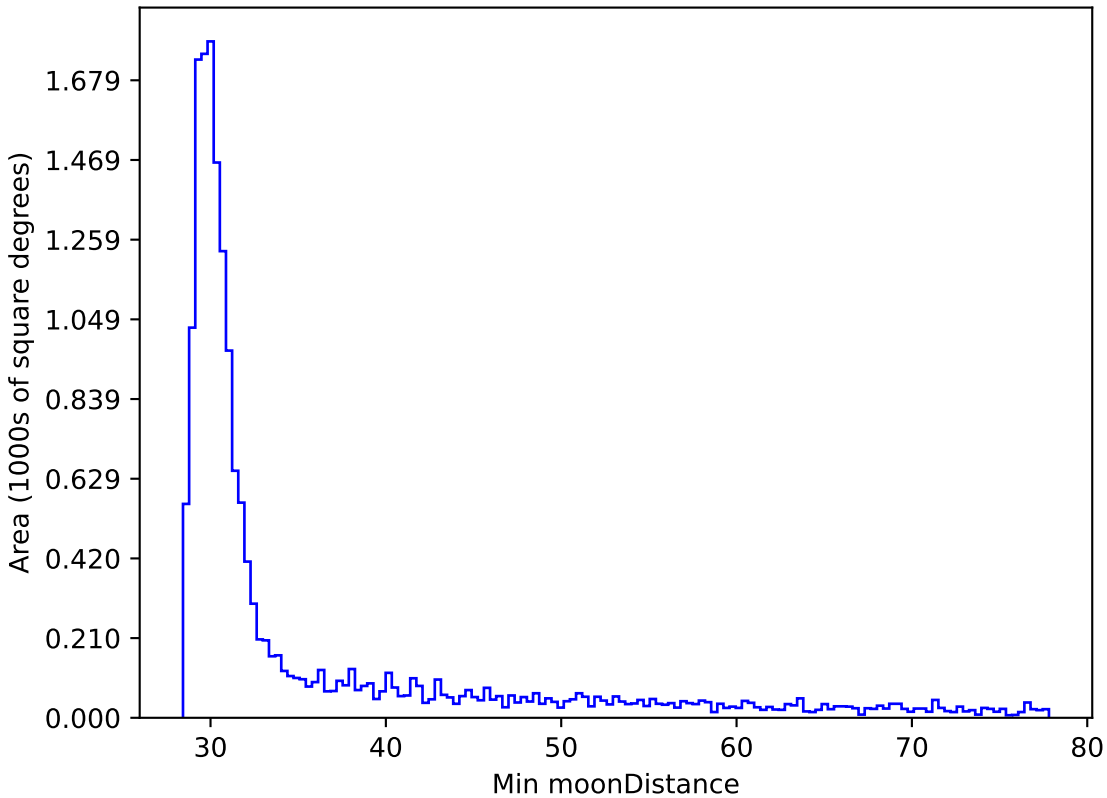
ddf_loaded_half_fl1_v3.4_10yrs WFD i band: Min moonDistance
