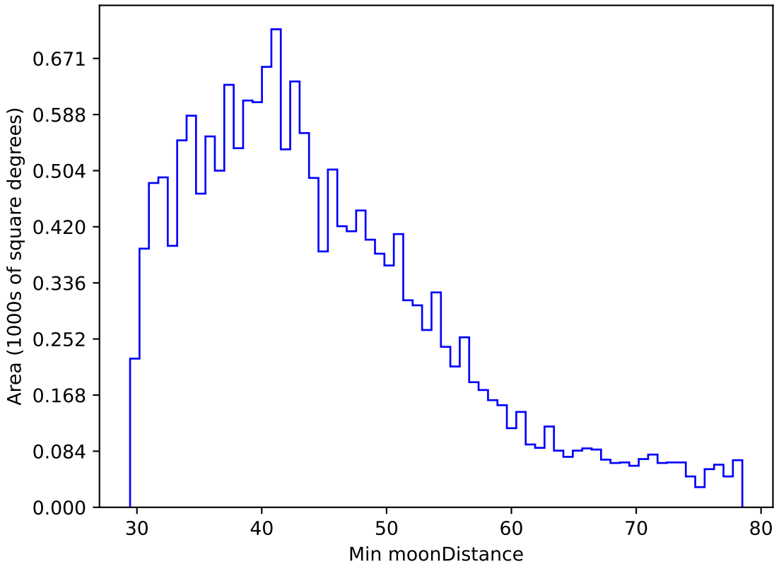
ddf_loaded_half_fl1_v3.4_10yrs WFD g band: Min moonDistance
