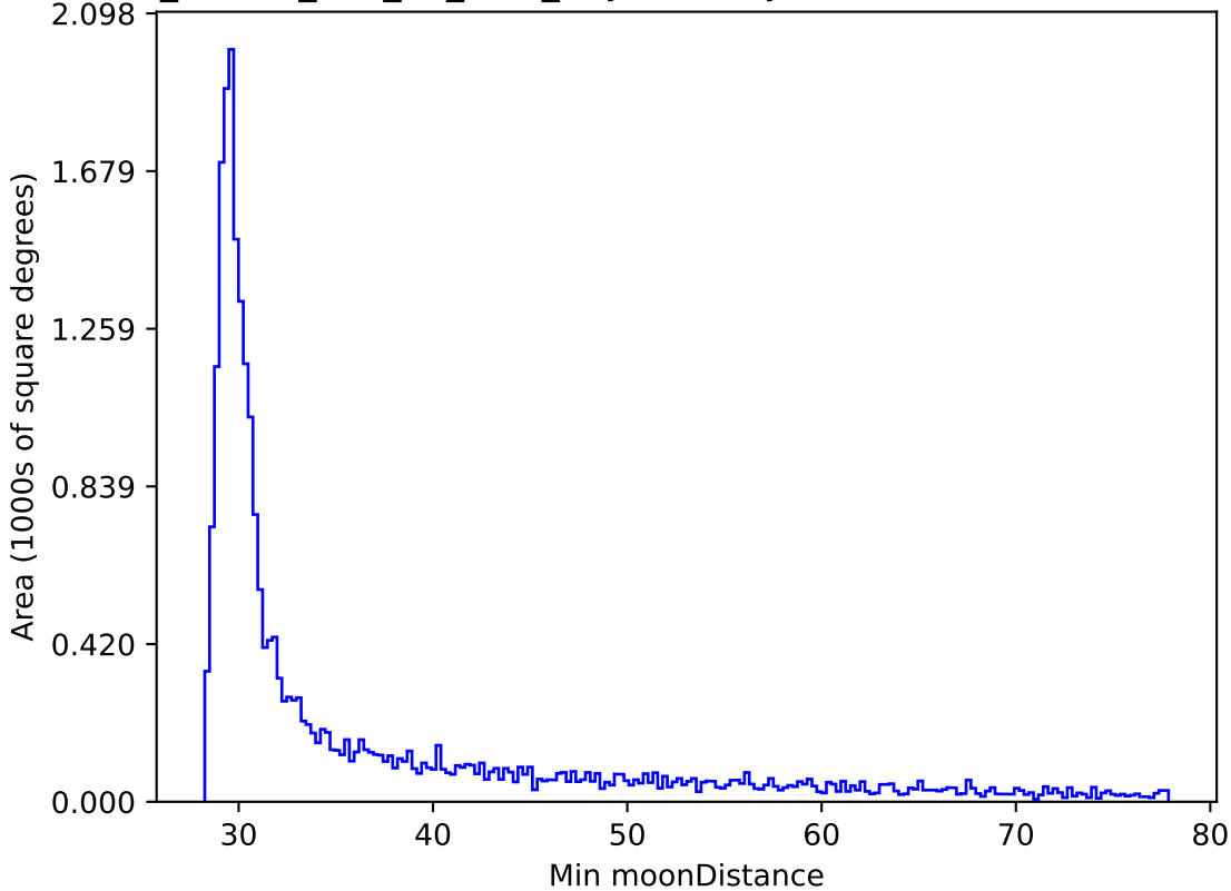
ddf_loaded_half_fl1_v3.4_10yrs All sky z band: Min moonDistance
