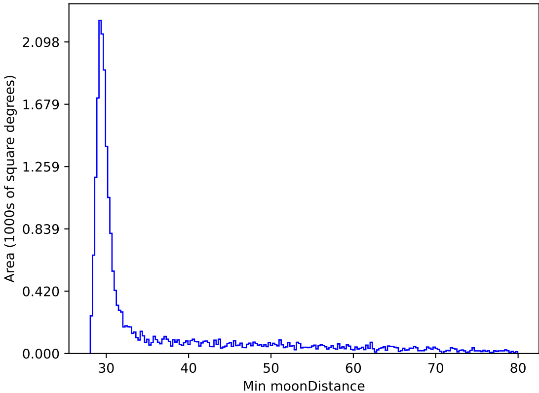
ddf_loaded_half_fl1_v3.4_10yrs All sky y band: Min moonDistance
