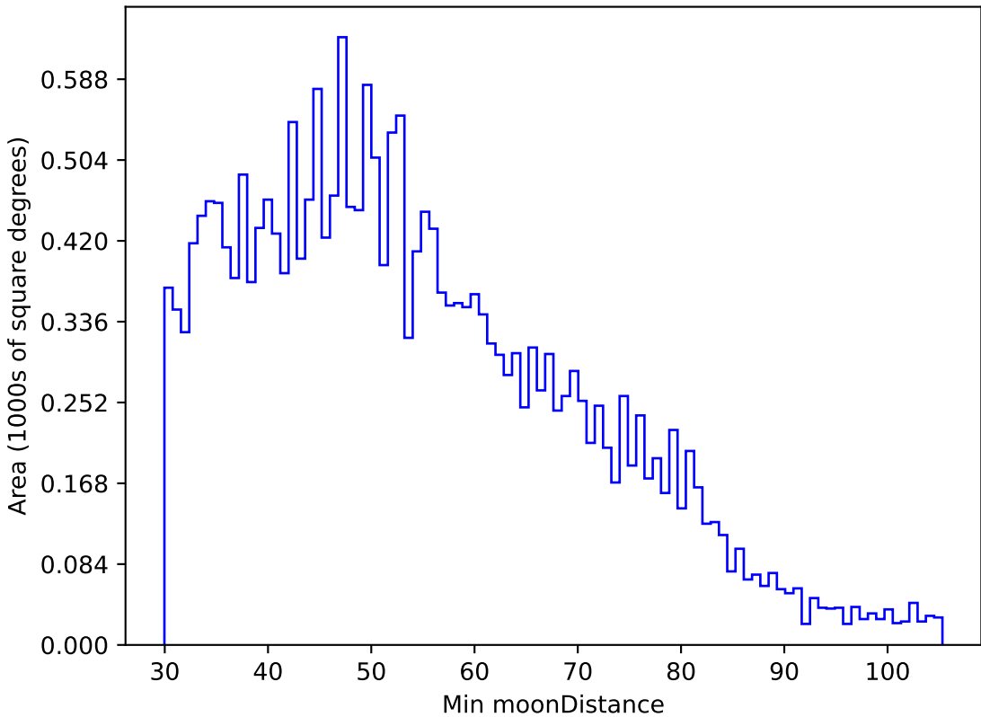
ddf_loaded_half_fl1_v3.4_10yrs All sky u band: Min moonDistance
