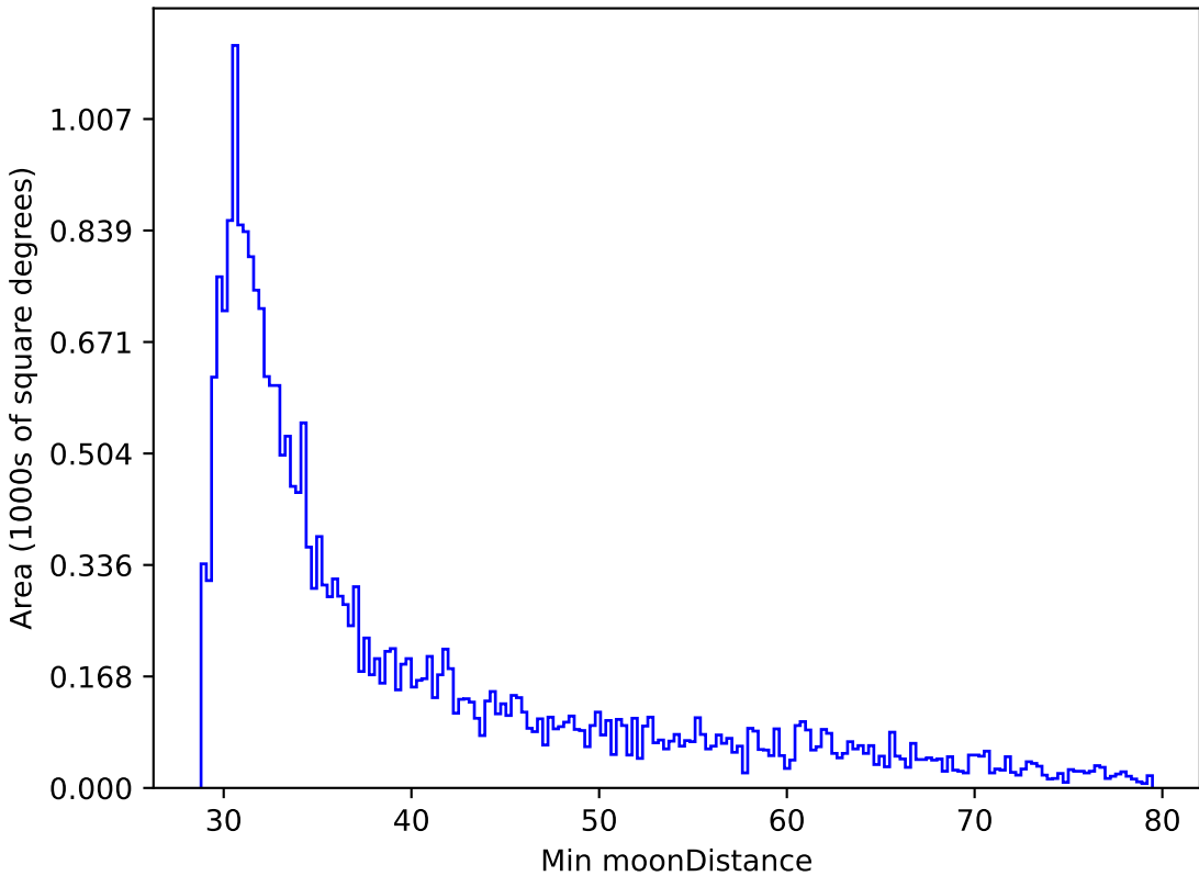
ddf_loaded_half_fl1_v3.4_10yrs All sky r band: Min moonDistance
