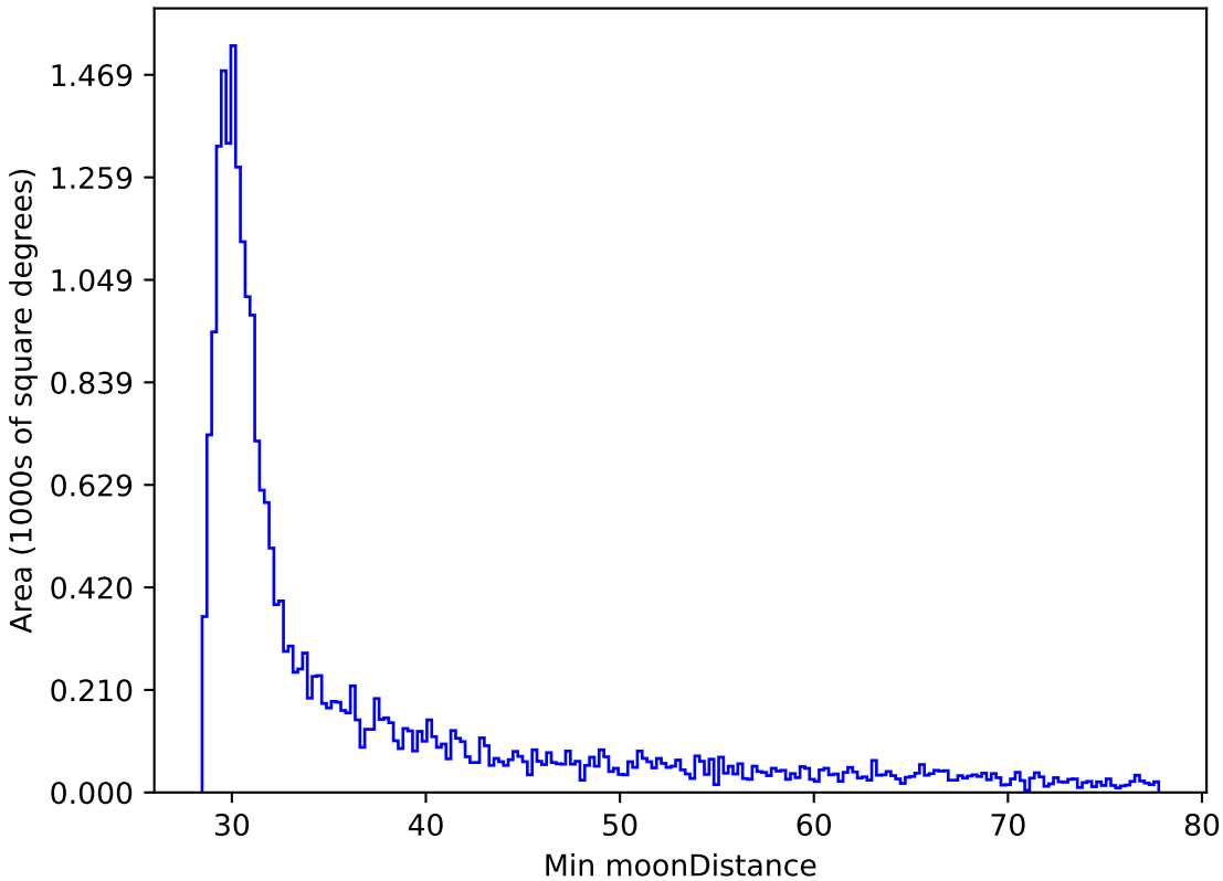
ddf_loaded_half_fl1_v3.4_10yrs All sky i band: Min moonDistance
