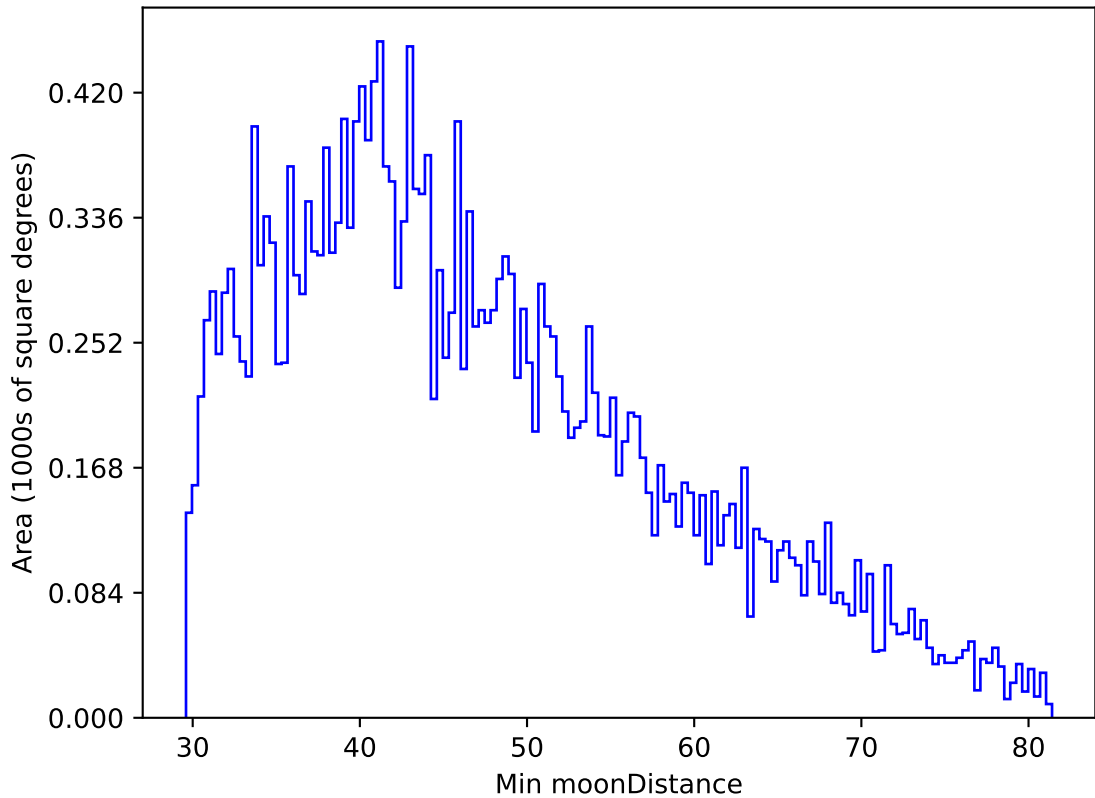
ddf_loaded_half_fl1_v3.4_10yrs All sky g band: Min moonDistance
