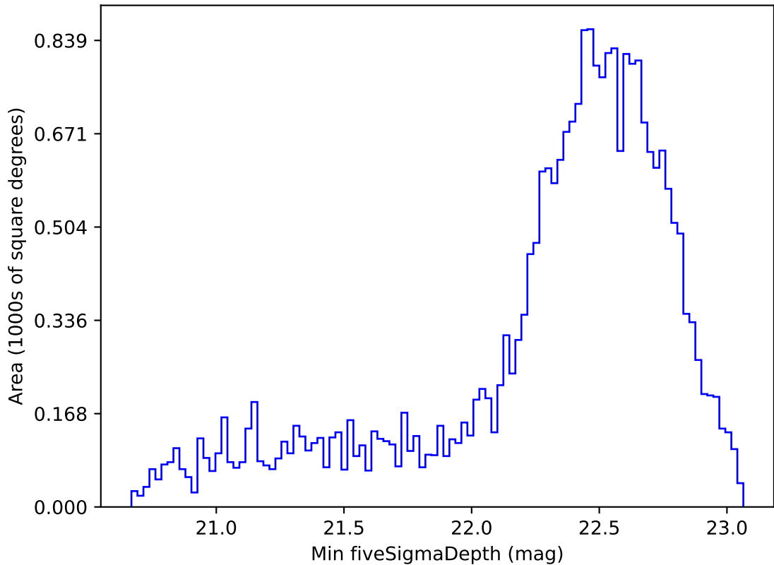
ddf_loaded_half_fl1_v3.4_10yrs Yr 1 z band: Min fiveSigmaDepth
