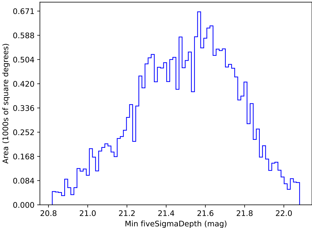
ddf_loaded_half_fl1_v3.4_10yrs Yr 1 y band: Min fiveSigmaDepth
