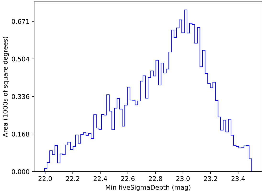
ddf_loaded_half_fl1_v3.4_10yrs Yr 1 u band: Min fiveSigmaDepth
