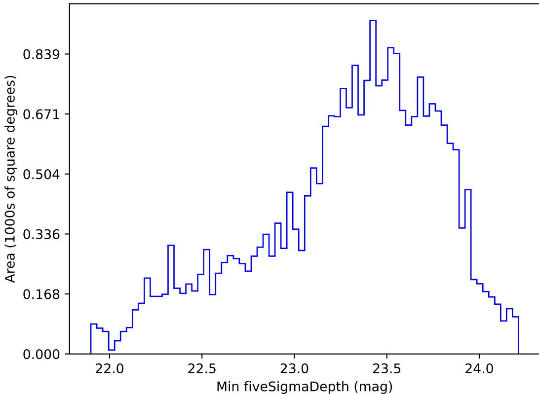
ddf_loaded_half_fl1_v3.4_10yrs Yr 1 r band: Min fiveSigmaDepth
