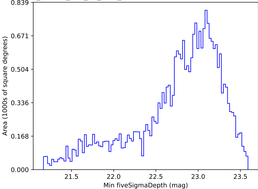
ddf_loaded_half_fl1_v3.4_10yrs Yr 1 i band: Min fiveSigmaDepth
