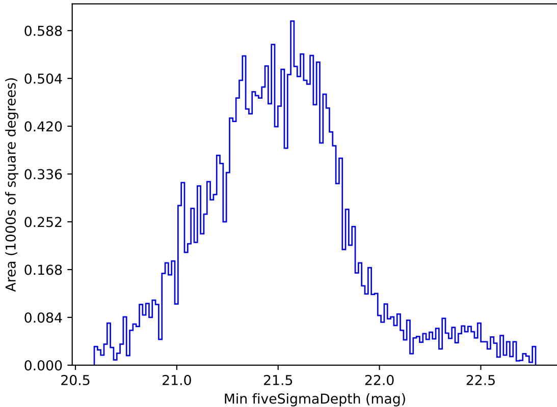
ddf_loaded_half_fl1_v3.4_10yrs Yr 1 all bands: Min fiveSigmaDepth
