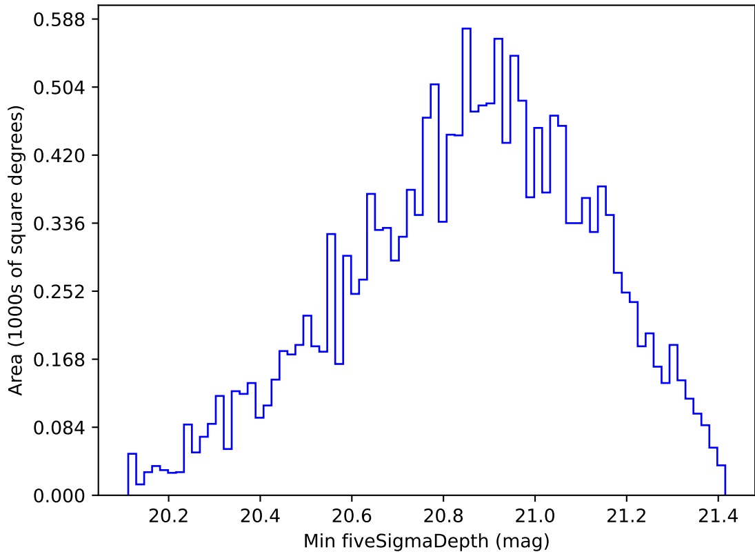
ddf_loaded_half_fl1_v3.4_10yrs WFD y band: Min fiveSigmaDepth
