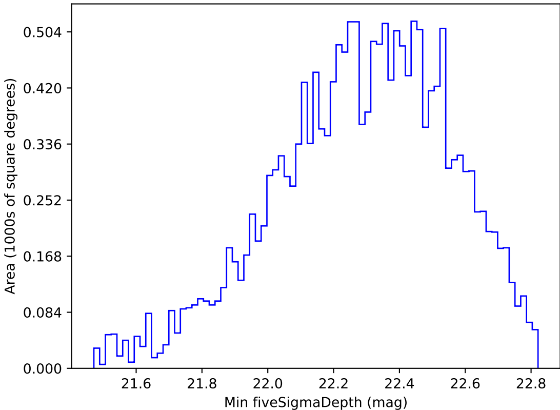
ddf_loaded_half_fl1_v3.4_10yrs WFD u band: Min fiveSigmaDepth
