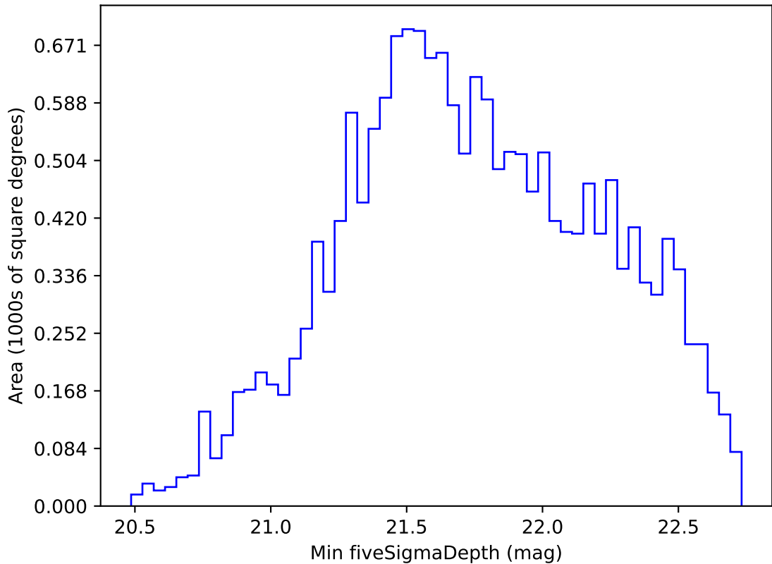
ddf_loaded_half_fl1_v3.4_10yrs WFD i band: Min fiveSigmaDepth
