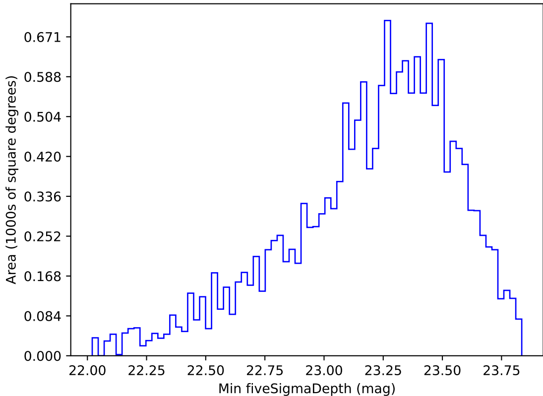
ddf_loaded_half_fl1_v3.4_10yrs WFD g band: Min fiveSigmaDepth
