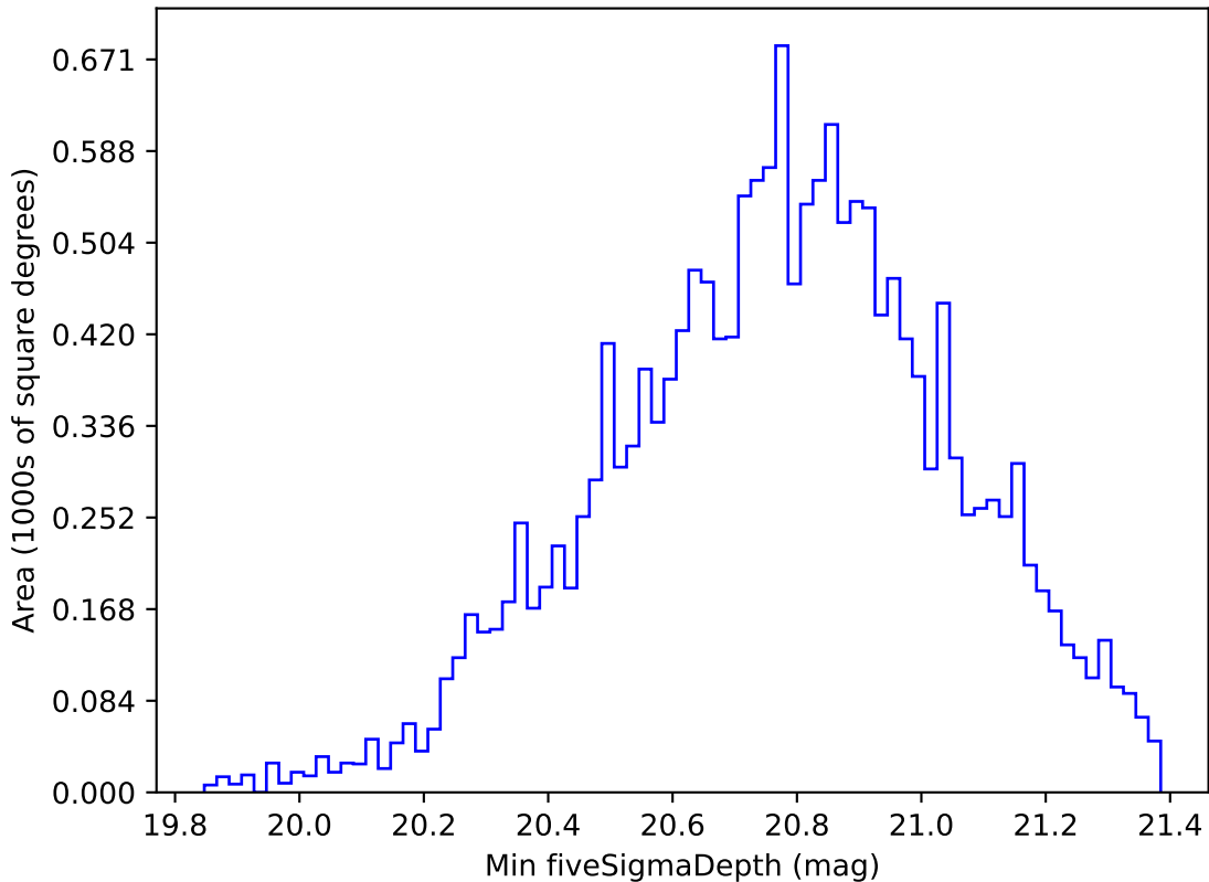
ddf_loaded_half_fl1_v3.4_10yrs WFD all bands: Min fiveSigmaDepth
