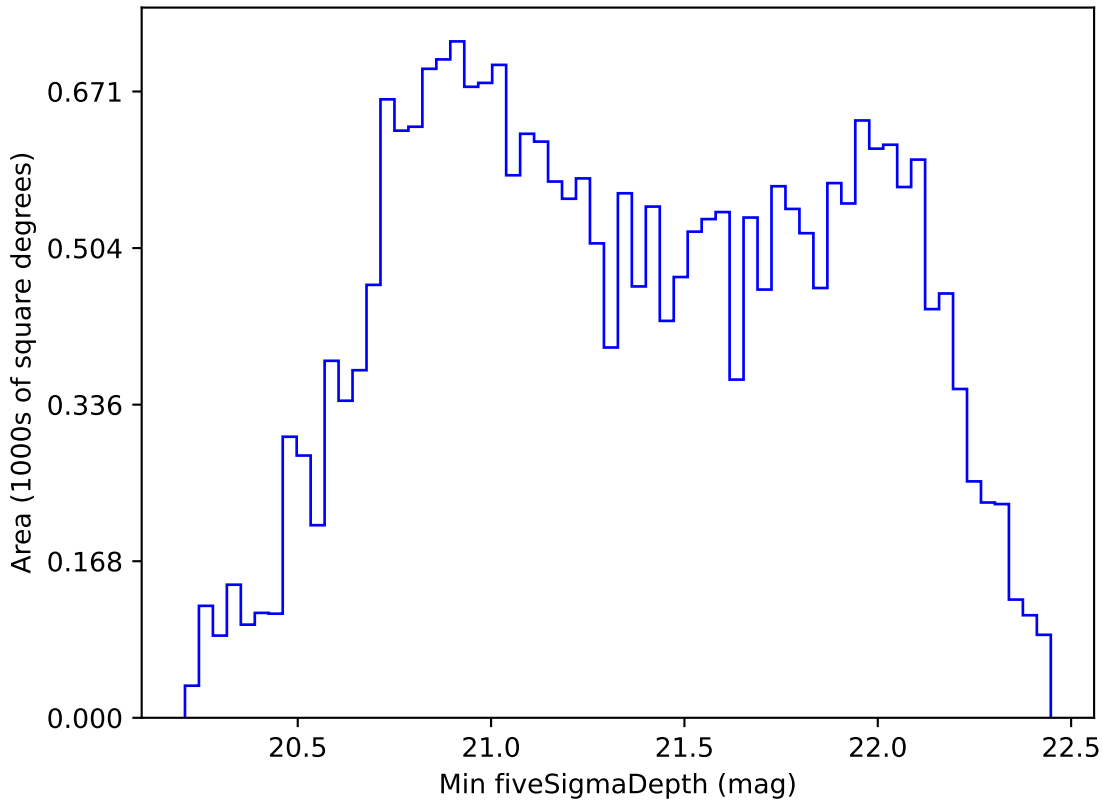
ddf_loaded_half_fl1_v3.4_10yrs All sky z band: Min fiveSigmaDepth
